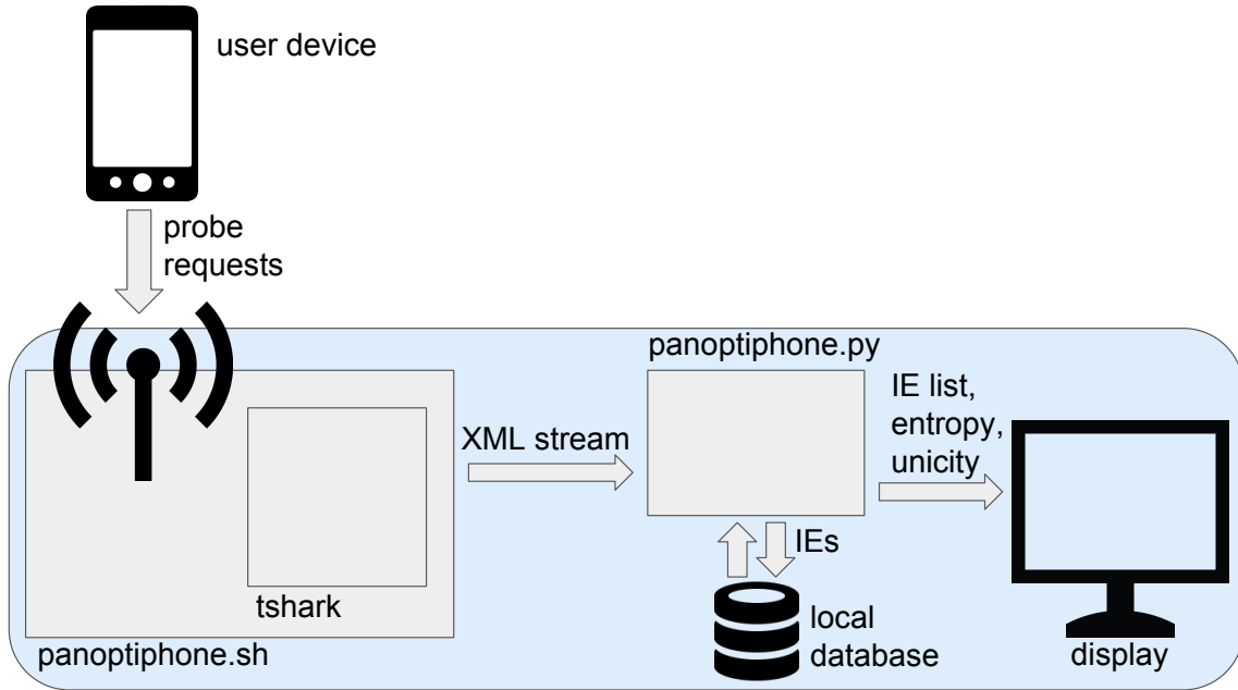
Figure V.3 – Architecture of the Panoptiphone system.
